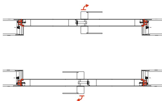
INSTALLATION PULL EU LEFT
