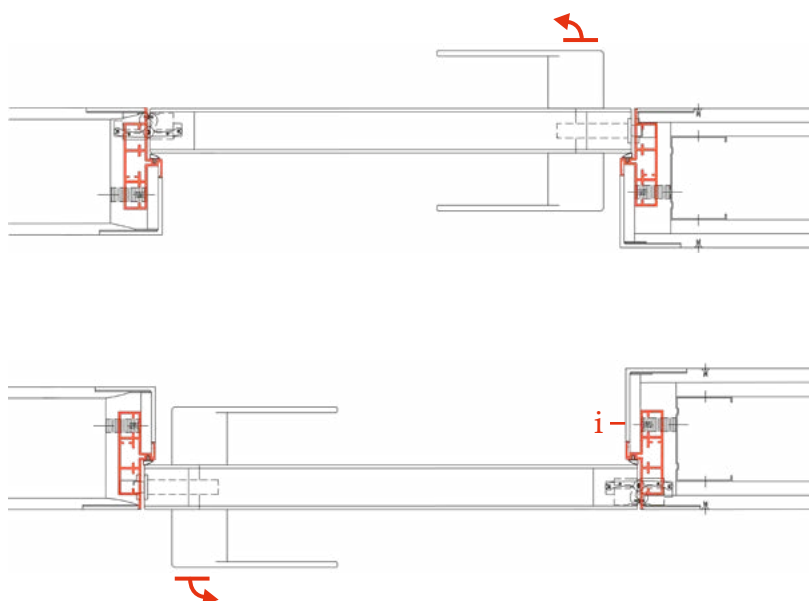
INSTALLATION PULL EU RIGHT
