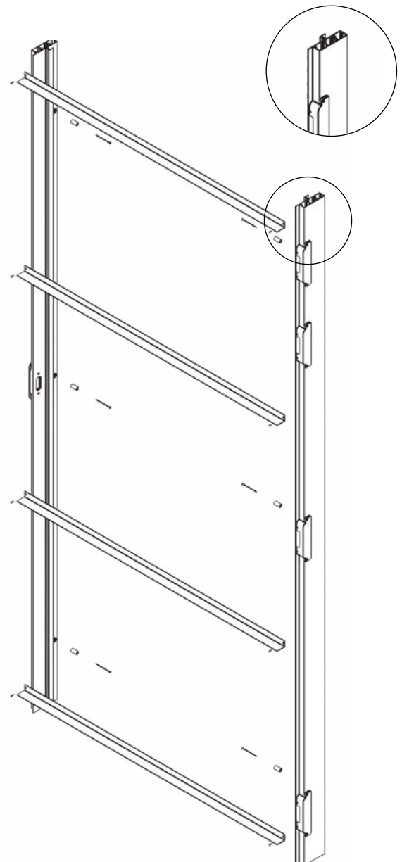
FRAME TYPE C - 90° FRAME
