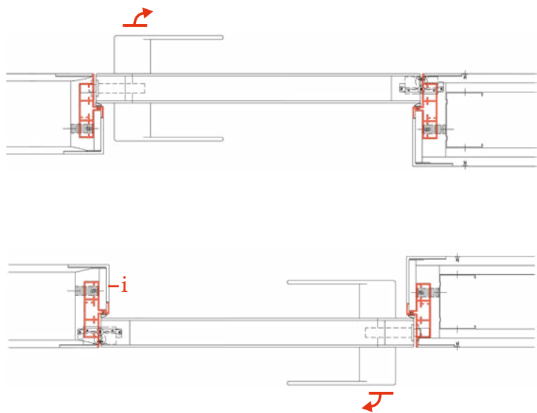
INSTALLATION PULL EU LEFT
